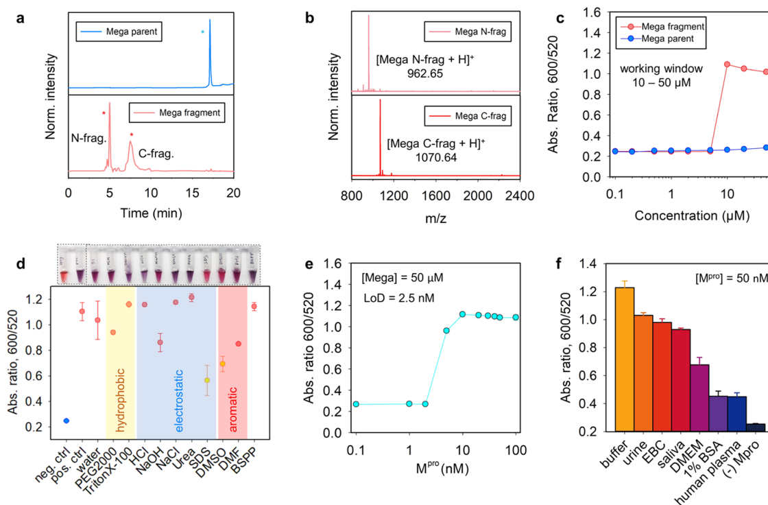
Figure 5. Improved performance of Mega peptide in colorimetric sensor. (a, b) HPLC and ESI-MS data confirm that M^{pro} cleaves the Mega peptide between Q and S. Peaks with * are the intact peptide (blue); the fragments are in red. (c) Ratiometric signal ( Abs_{600}/Abs_{520} at 10 min readout time) recorded from BSP- AuNPs ( 3.4\text{ nM} , 100\ \mu\text{L} ) incubated with various amounts of intact Mega (red) and the fragments (blue). (d) White-light image (top) and quantified reversal color change (bottom) of the Mega/ AuNP pellet in different surfactant solutions ( 10\text{ mM} , 100\ \mu\text{L} ) or solvents ( 100\ \mu\text{L} ). The redispersion in an SDS solution and DMSO solvent indicates dominant electrostatic and aromatic forces with scarce covalent bonding. (e) Ratiometric absorbance as a function of M^{pro} concentration. Conditions used the Mega substrate ( 100\ \mu\text{M} ), BSP- AuNPs ( 3.4\text{ nM} ), and a 10 min assay time. The determined limit of detection is 2.5\text{ nM} in Tris buffer. (f) Sensor performance in other biological media. Positive control used the buffer with M^{pro} ( 100\text{ nM} ), and negative control used the buffer without M^{pro} . Error bar = standard deviation ( n = 3 ).
