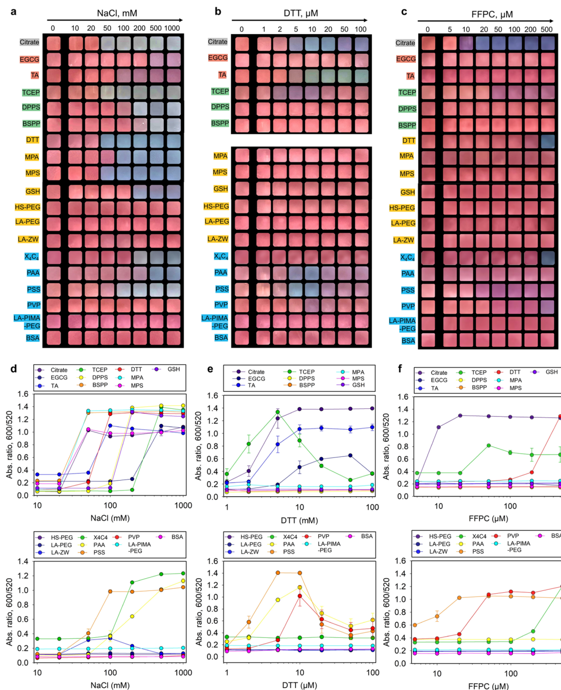
Figure 3. (a–c) Color patterns of the ligated AuNPs (3.4 nM, 100 μL) in a series of NaCl, dithiothreitol (DTT), and amphiphilic peptide (FFPC) solutions of increasing concentrations (pH ~8.0). Shown are the cropped images at 10 min incubation. Red indicates dispersed nanoparticles. Purple, blue, and gray indicate increasing aggregation levels. The color pattern of DTT-AuNPs under DTT test is not included due to low reproducibility. (d–f) Quantitative analysis of the color patterns by measuring the ratiometric absorbance, \text{Abs}_{600}/\text{Abs}_{520} . The critical coagulation concentration (CCC) is defined as the first point of signal jump, where the ratiometric absorbance may vary. Error bars = standard deviations ( n = 3 ). Panel (b) is reprinted with permission from ref 16. Copyright 2022 American Chemical Society.
